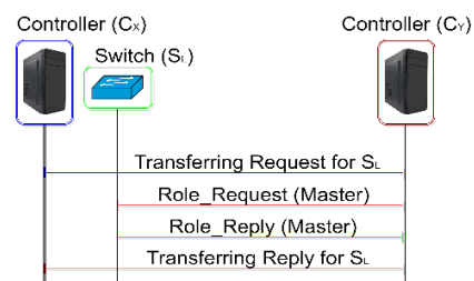
Figure 2. Switch transferring process in OpenFlow Protocol.
