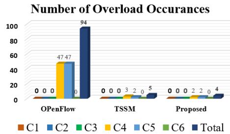
Figure 6. Comparison of number of overload occurrences in conventional and proposed method.
